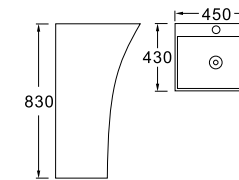
LX-8016 Vitreous China 450x430x830mm Fixing to wall with back
