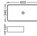
LX-7342 Vitreous China 600x340x110mm Above counter mounting
