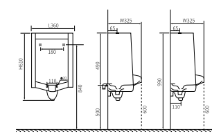
LX-3141 Wall-hanging Type Vitreous China 360x325x610mm
