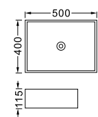
LX-7071 Vitreous China 500x400x115mm Above counter mounting
