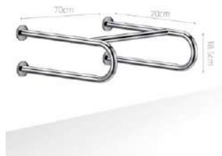
LX-H002 handrail SUS304 Ø32mm
