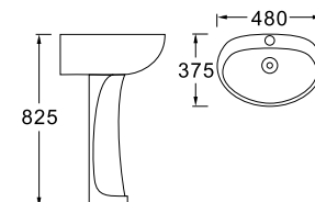
LX-3209F Vitreous China 480x375x825mm Fixing to wall with back
