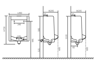
LX-3108 Wall-hanging Type Vitreous China 490x295x730mm
