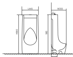
LX-3105 Floor type Vitreous China 445x355x980mm
