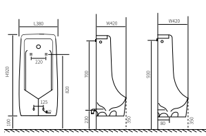
LX-3157 Wall-hanging Type Vitreous China 380x420x920mm
