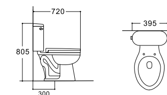
LX-2756B Siphonic Flushing Vitreous China 720x395x805mm S-trap 300mm
