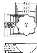
LX-0009 Vitreous China 420x420x140mm 380x380x130mm 350x350x130mm 310x310x120mm Above counter mounting
