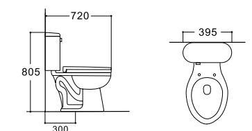
LX-2756C Siphonic Flushing Vitreous China 720x395x805mm S-trap 300mm
