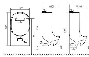
LX-3126 Wall-hanging Type Vitreous China 360x305x650mm
