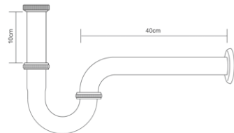
LX-P03 Drain-Pipe SUS201 Chrome
