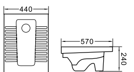
LX-3824S Squatting Pan W.C Vitreous China 570x440x240mm Fixing ti wall with back
