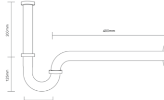
LX-P05M Drain-Pipe SUS304 Satin Finish
