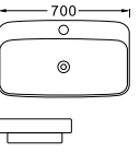
LX-5437 Vitreous China 700x420x155mm Above counter mounting
