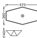
LX-5615 Vitreous China 570x360x140mm Above counter mounting
