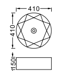
LX-8449P-6 Vitreous China 410x410x150mm Above counter mounting
