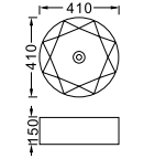
LX-8449P-4 Vitreous China 410x410x150mm Above counter mounting
