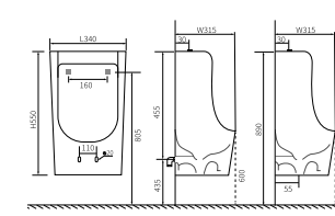
LX-3148 Wall-hanging Type Vitreous China 340x315x550mm
