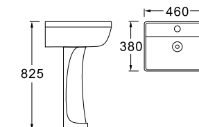
LX-5620F Vitreous China 460x380x825mm Fixing to wall with back
