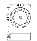
LX-8449P-7 Vitreous China 410x410x150mm Above counter mounting
