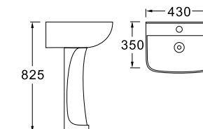
LX-3210F Vitreous China 430x350x825mm Fixing to wall with back
