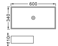
LX-7084 Vitreous China 600x340x110mm Above counter mounting
