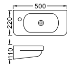
LX-5361 Vitreous China 500x220x110mm Hanging installation
