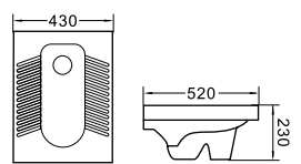
LX-3825S Squatting Pan W.C Vitreous China 520x430x230mm Fixing ti wall with back
