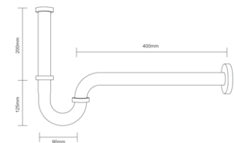
LX-P05 Drain-Pipe SUS304 Chrome
