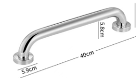
LX-H007 handrail SUS304 Ø32mm
