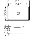
LX-5178A/B Vitreous China A: 650x350x140mm B: 545x350x125mm Above counter mounting
