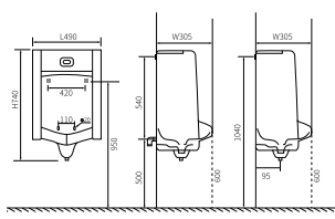
LX-3102 Wall-hanging Type Vitreous China 490x305x740mm
