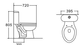
LX-2756A Siphonic Flushing Vitreous China 720x395x805mm S-trap 300mm
