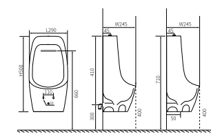
LX-3410 Wall-hanging Type Vitreous China 290x245x500mm
