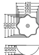
LX-0008 Vitreous China 420x420x140mm 380x380x130mm 350x350x130mm 310x310x120mm Above counter mounting
