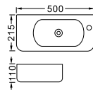
LX-5362 Vitreous China 500x215x110mm Hanging installation
